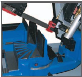
WE270DS Dual Direction Vice
